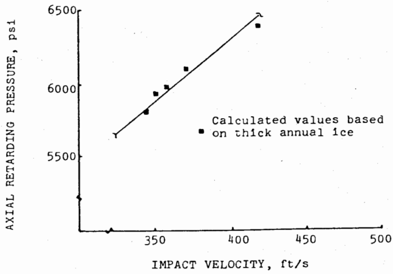
Figure 3. Axial Retarding Pressure on the Nose of a 15-inch Diameter System with a 2.2 CRH Nose at Various Impact Velocities
